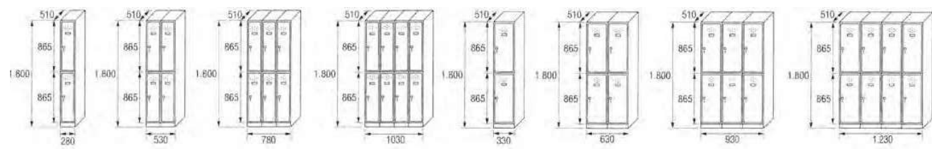
AT-25/1 COD. 32511 AT-25/2 COD. 32512 AT-25/3 COD. 32513 AT-25/4 COD. 32514 AT-30/1 COD. 33011 AT-30/2 COD. 33012 AT-30/3 COD. 33013 AT-30/4 COD. 33014
