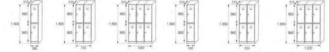
AT-35/1 COD. 33511 AT-35/2 COD. 33512 AT-35/3 COD. 33513 AT-40/1 COD. 34011 AT-40/2 COD. 34012 AT-40/3 COD. 34013
